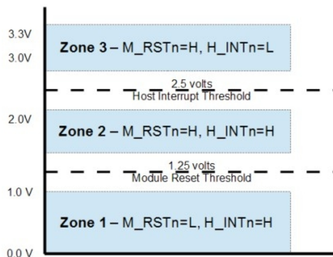
Figure 11: INT/RSTn Voltage Zones
