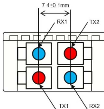
Figure 10: Module Optical Interface (looking into the optical port)
