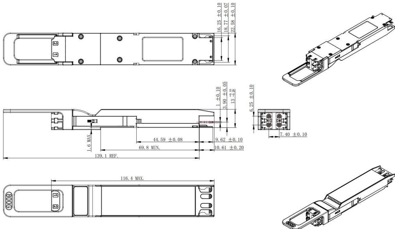
Figure 8: Mechanical Package Outline (All dimensions in mm)
