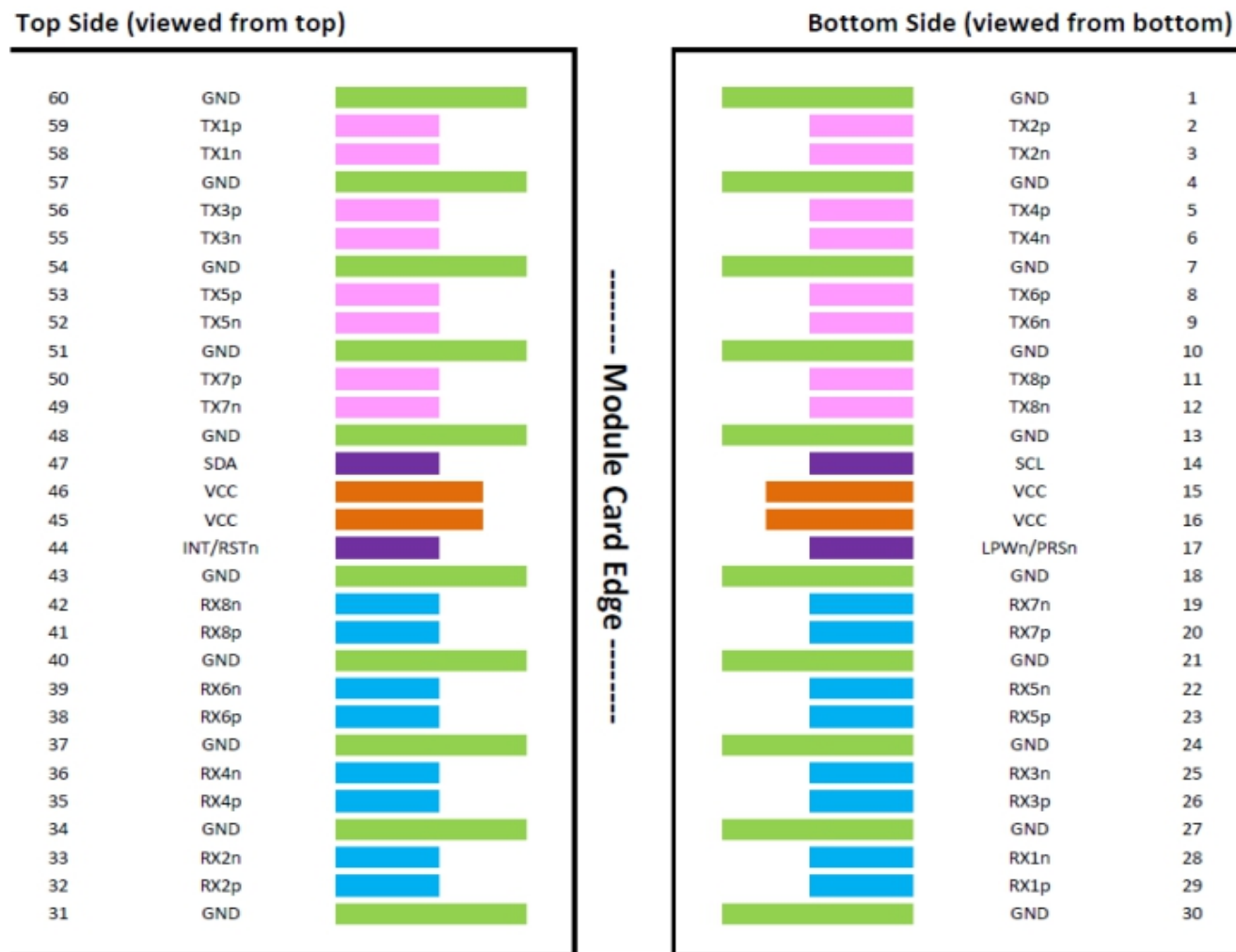
Figure 6: OSFP Module Pinout
