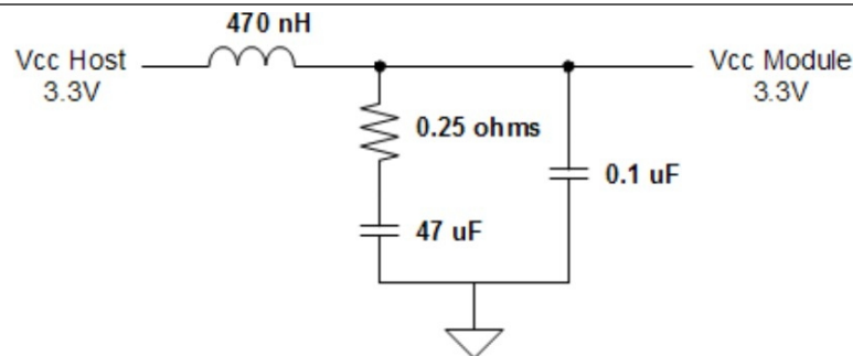
Figure 7: Recommended Host Board Power Supply Filter
