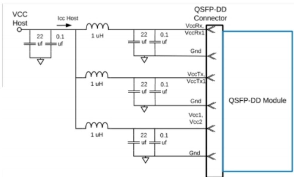
Figure 7: Host Board Power Supply Filter
