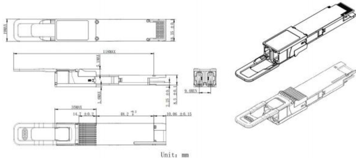
Figure 8: Mechanical Package Outline (All dimensions in mm)
