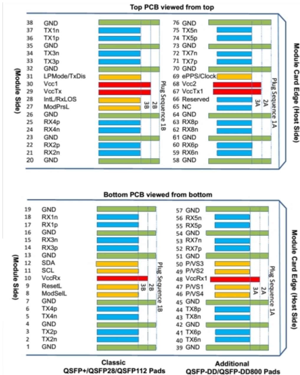
Figure 6: QSFP-DD Module Pinout
