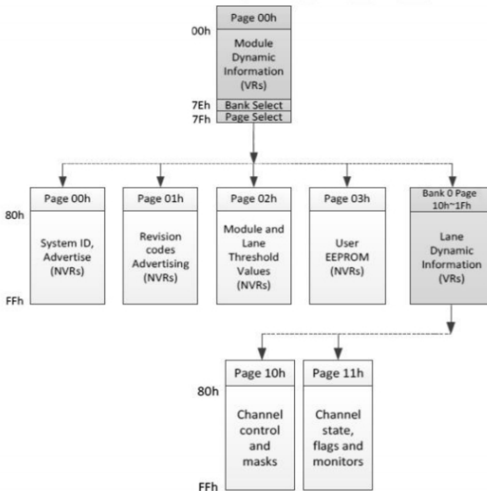
Figure 11: Simplified QSFP-DD CMIS Module Memory Map Architecture
