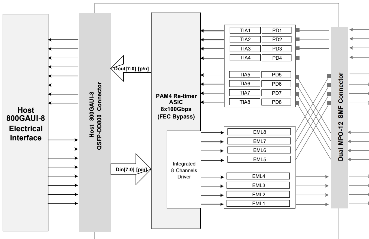
Figure 2: Application Reference Diagram
