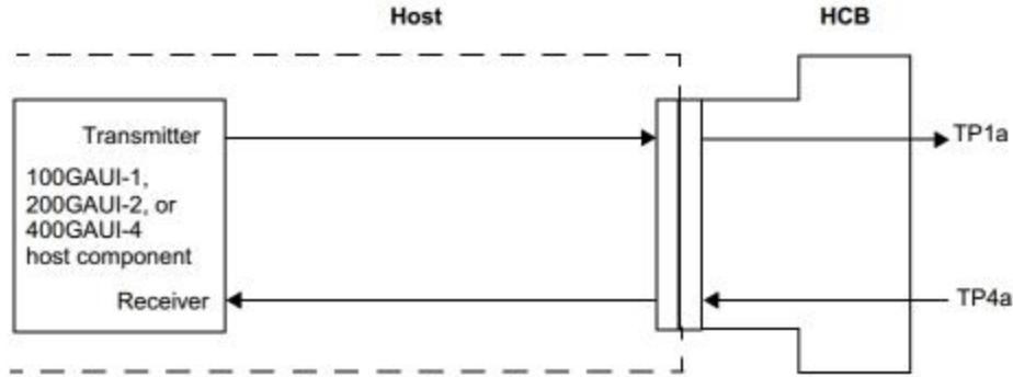
Figure 4: IEEE 802.3ck host compliance points TP1a, TP4a
