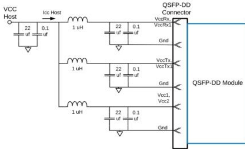
Figure 7: Host Board Power Supply Filter
