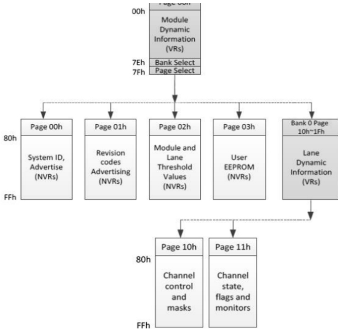
Figure 11: Simplified QSFP-DD CMIS Module Memory Map Architecture
