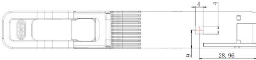
Figure 9: Case Temperature Measurement Point (All dimensions in mm)
