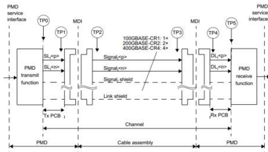
Figure 3: IEEE 802.3ck 100GBASE-CR1, 200GBASE-CR2 or 400GBASE-CR4 link
