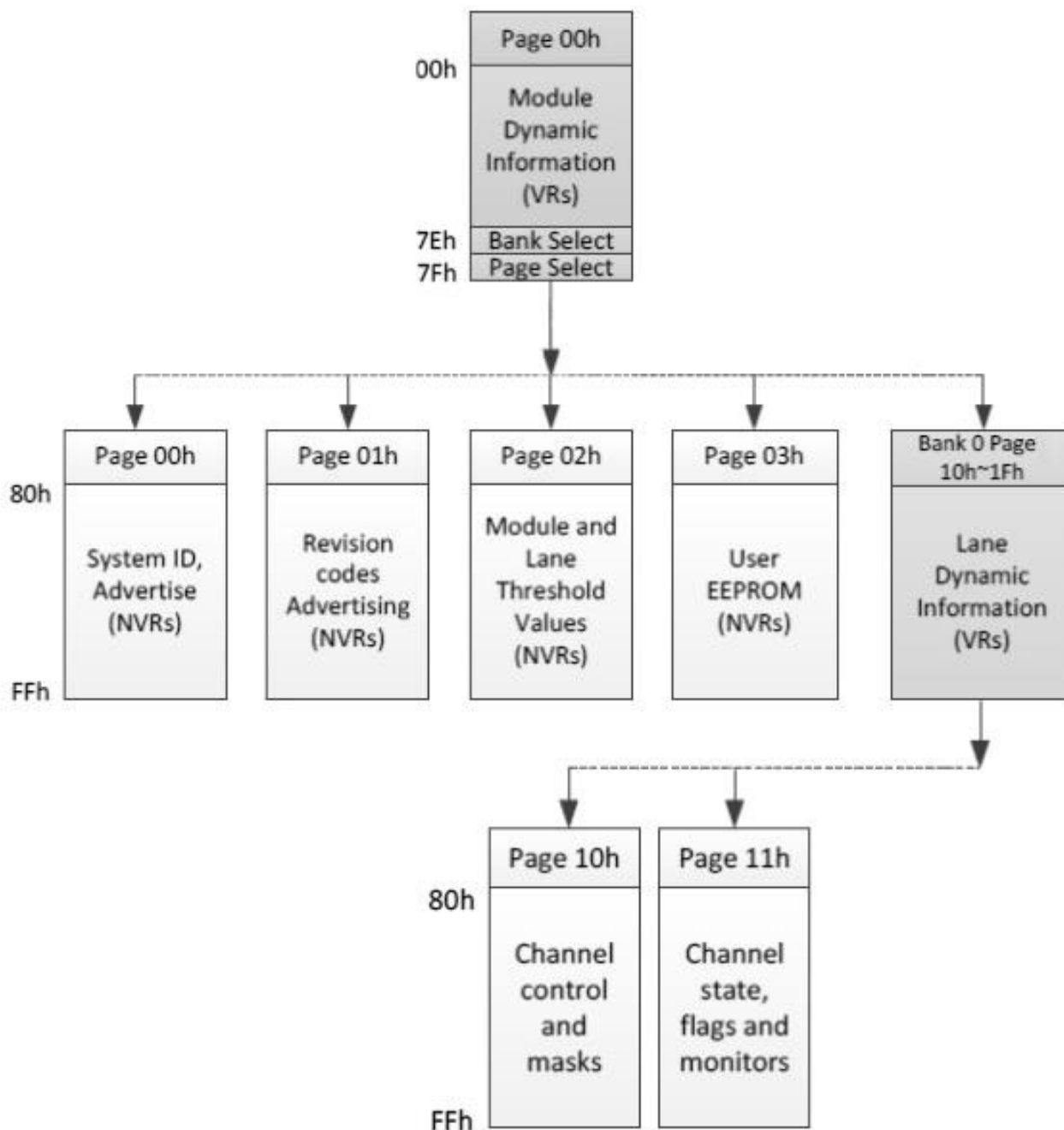
Figure 13: Simplified QSFP-DD CMIS Module Memory Map Architecture
